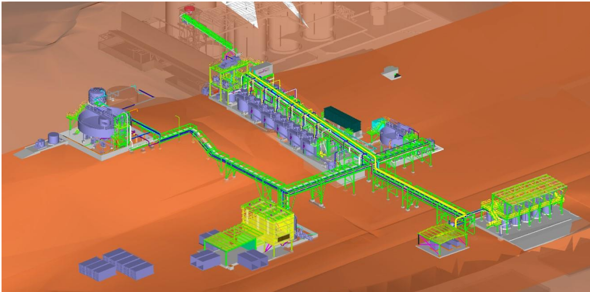
Figure 2: Finalized 3D Model of Sulphide Flotation Circuit Addition to Selinsing Gold Plant
